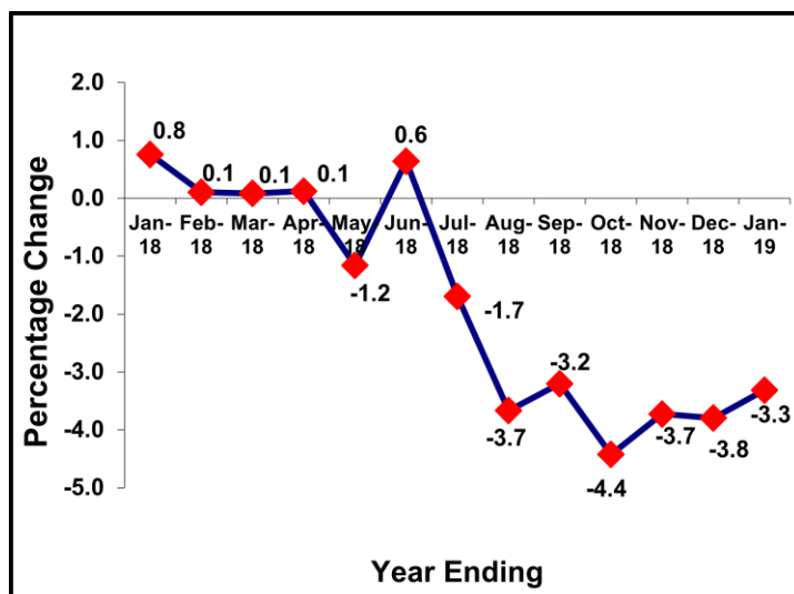
Figure 2: Annual changes in PPI-Manufacturing Jan 2018 – Jan 2019
