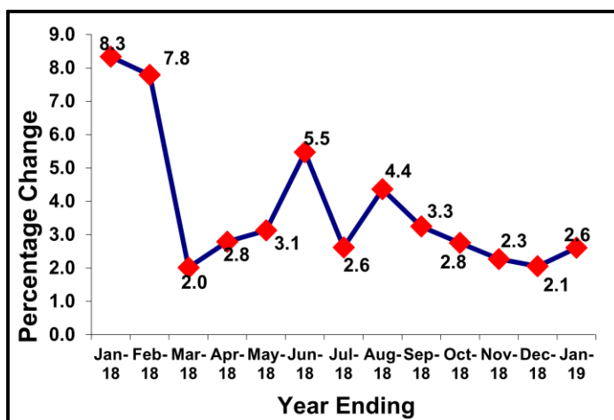
Figure 4: Annual changes in PPI-Utility Jan 2018 – Jan 2019
