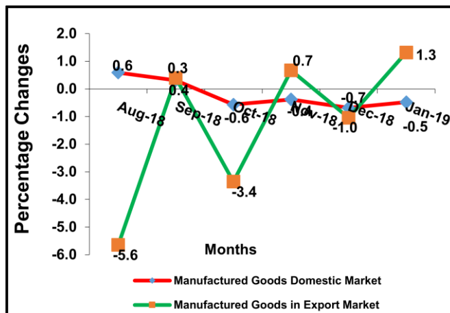
Figure 3: Monthly Changes in PPI-M, Domestic and Export August 2018 –January 2019
