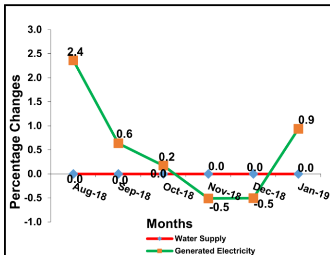
Figure 5: Monthly Changes in PPI-Utility August 2018 –January 2019
