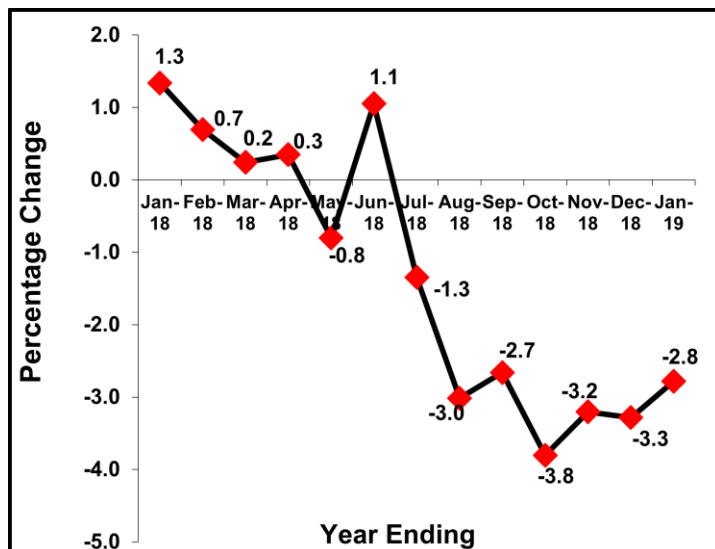
Figure 1: Annual changes in PPI-M&U January 2018 – January 2019
