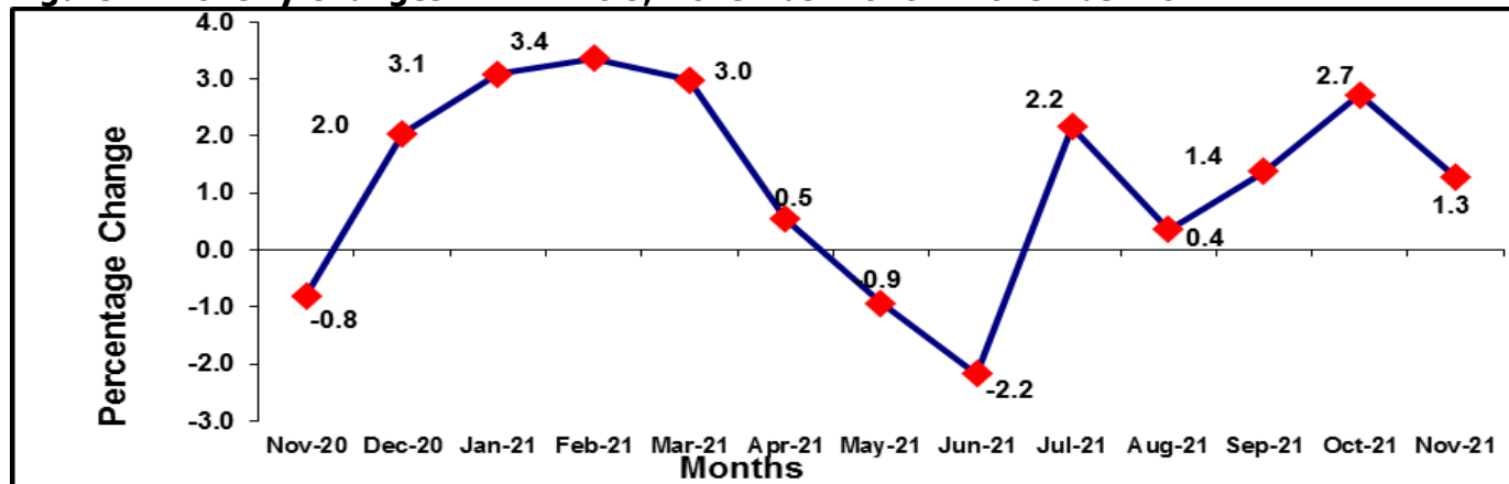
Figure 2: Monthly Changes in PPI-M&U, November 2020 – November 2021
