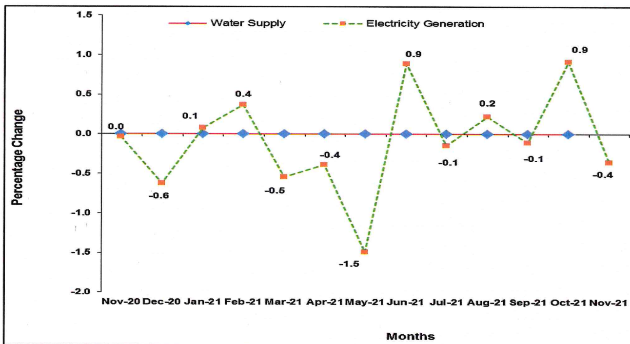
Figure 4: Monthly Changes in PPI-Utility, Water Supply and Electricity Generation November2020 – November2021
