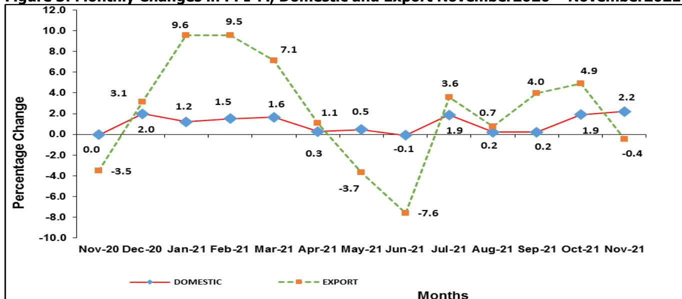
Figure 3: Monthly Changes in PPI-M, Domestic and Export November 2020 – November 2021
