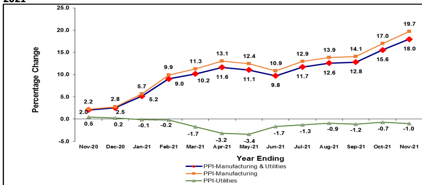
Figure 1: Annual percentage changes in Producer Price Indices, November 2020 – November 2021
