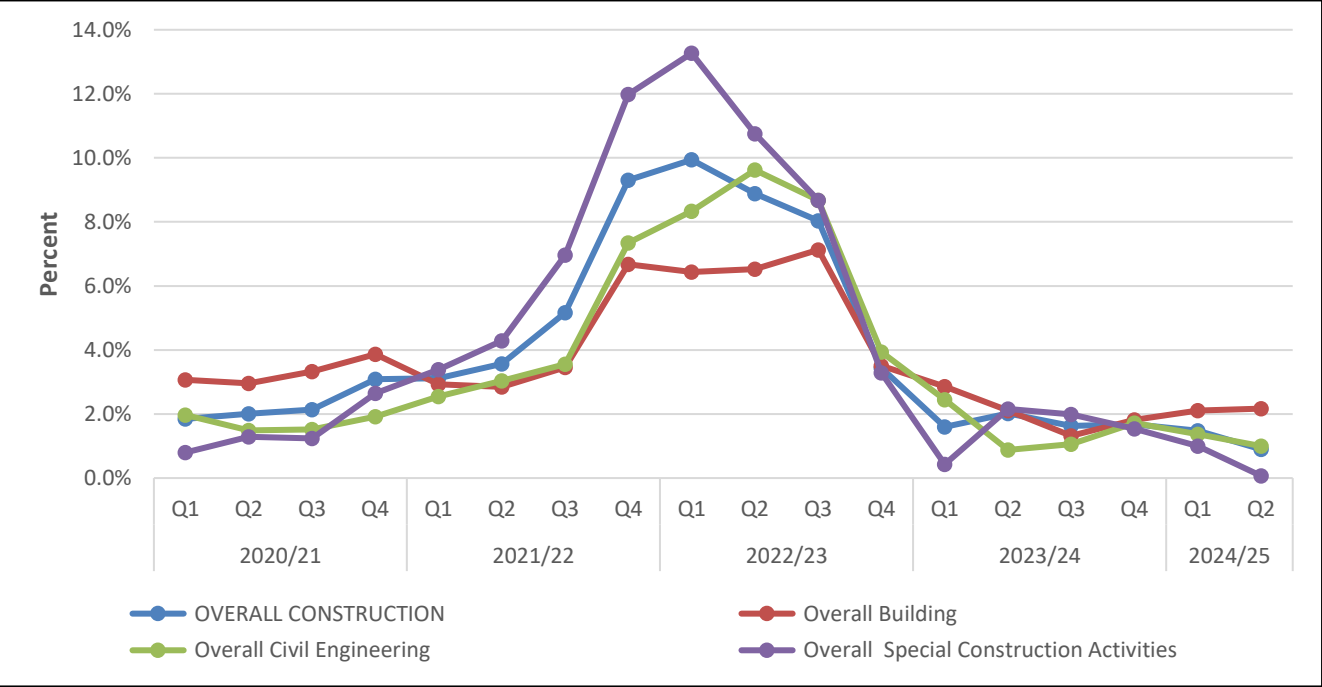
Figure 7: Construction Input Price Index, Annual percentage changes, Q1 2020/21 – Q2 2024/25
