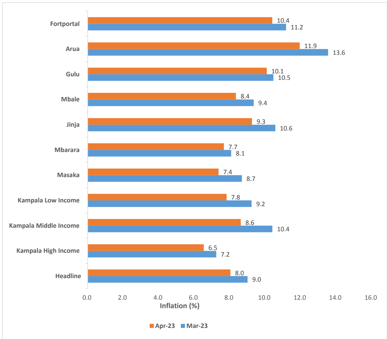
Figure 2: Annual Inflation by Income Groups and Geographical Areas for the 12 months to March 2023 and April 2023
