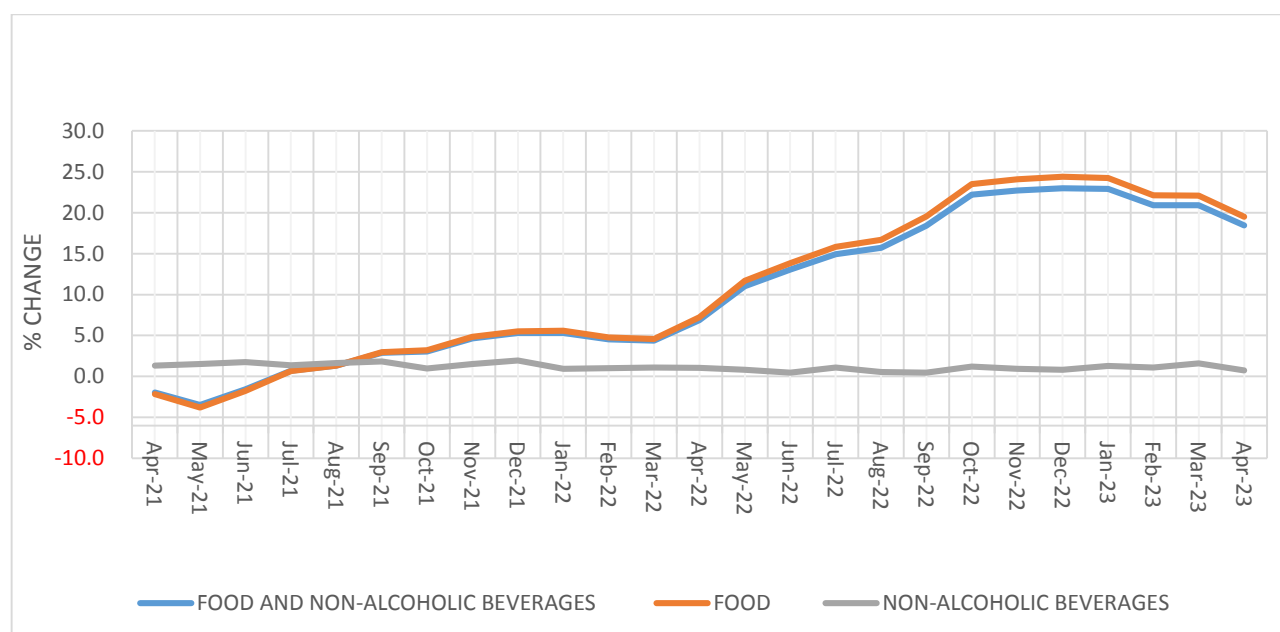
Figure 4: Food and Non Alcoholic Beverages Annual Inflation Trends; April 2021 – April 2023.
