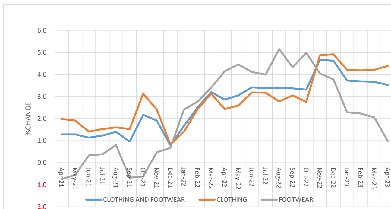
Figure 5: Clothing and Footwear Annual Inflation Trends; April 2021 – April 2023.
